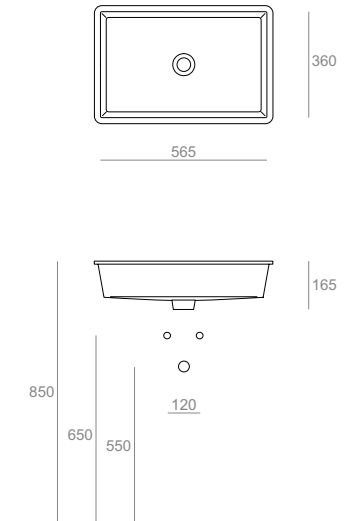
S60 Lavabo 55 sottopiano Undercoat washbasin 55 55.35.16
