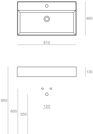
AG81 Lavabo 81 monoforo da appoggio o sospeso Countertop or wall-hung washbasin 81 for single tap hole 81.46.13
