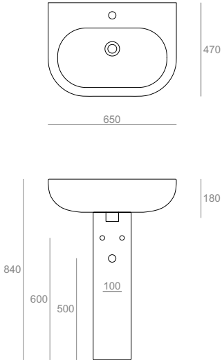
EL05 Lavabo 65 monoforo sospeso o su colonna (CN200) Washbasin 65 wall-hung or on pedestal (CN200) with for single tap hole 65.47.18
