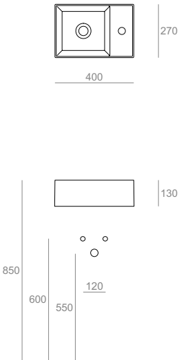
AG40 Lavamani 40 da appoggio o sospeso monoforo - mensola a dx Countertop or wall-hung hand washbasin 40 for single tap hole - right shelf 40.27.13
