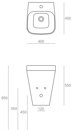
BB13 Lavabo 40.h55 sospeso monoforo Wall-hung washbasin 40.h55 for single tap hole 40.45.55
