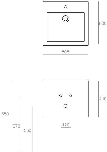
FZ13 Lavabo 50 sospeso predisposto monoforo Wall-hung washbasin 50 pre-punched for single tap hole 50.5.50.41
