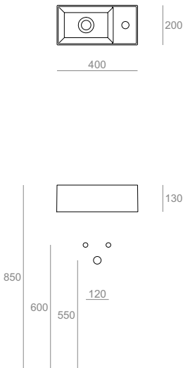
AG20 Lavamani 40 da appoggio o sospeso monoforo - mensola a dx Countertop or wall-hung hand washbasin 40 for single tap hole - right shelf 40.20.13
