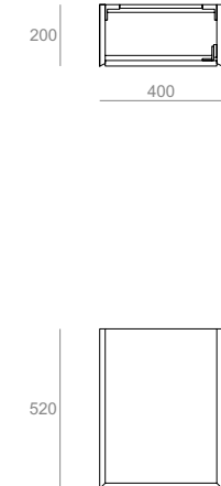
AGM20 Mobile sospeso per lavamani AG 20 con anta Wall-hung cabinet with door for hand washbasin AG 20 40.20.52
