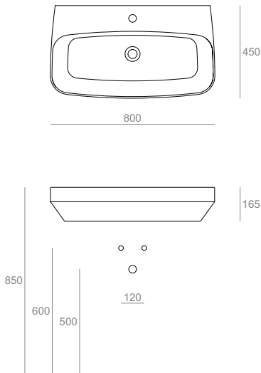
BB12 Lavabo 80 da appoggio o sospeso monoforo Countertop or wall-hung washbasin 80 for single tap hole 80.45.16
