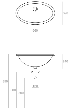
LFT74 Lavabo 66 ovale sottopiano Oval under-counter washbasin 66 66.39.24
