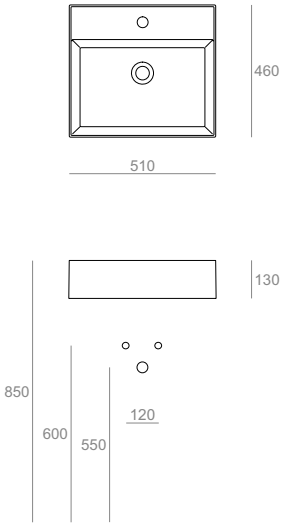
AG51 Lavabo 51 monoforo da appoggio o sospeso Countertop or wall-hung washbasin 51 for single tap hole 51.46.13
