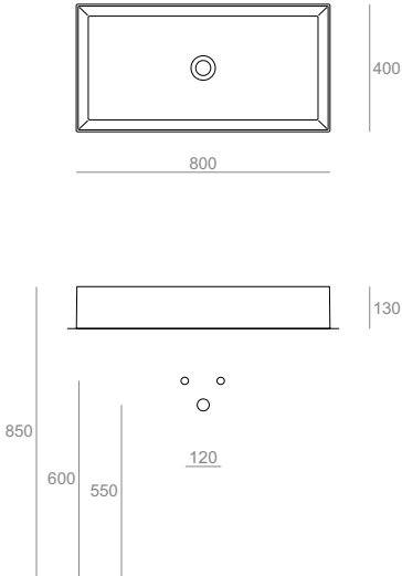
AG80 Lavabo 80 da appoggio Countertop washbasin 80 80.40.13
