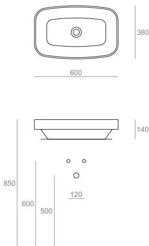
BB11 Lavabo 60 da appoggio e incasso Countertop and fully inset washbasin 60 60.38.14
