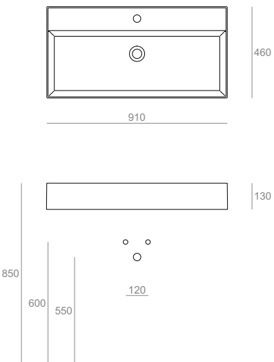
AG91 Lavabo 91 monoforo da appoggio o sospeso Countertop or wall-hung washbasin 91 for single tap hole 91.46.13
