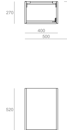
AGM40 - AGM50 Mobile sospeso per lavamani AG 40 - AG 50 con anta Wall-hung cabinet with door for hand washbasin AG 40 - AG 50 40.27.52 - 50.27.52
