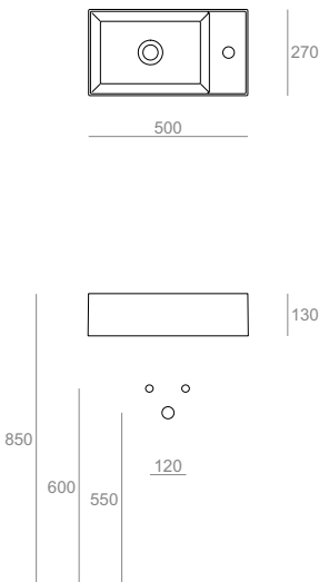
AG50 Lavamani 50 da appoggio o sospeso monoforo - mensola a dx Countertop or wall-hung hand washbasin 50 for single tap hole - right shelf 50.27.13
