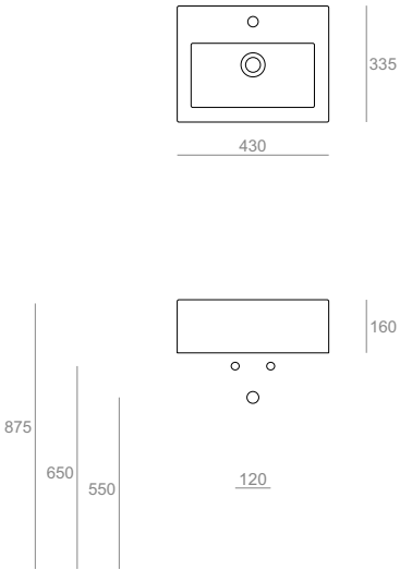
FZ14 Lavamani 43 sospeso predisposto monoforo Wall-hung hand washbasin 43 pre-punched for single tap hole 43.33.5.16
