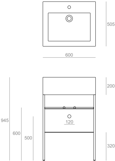
Mensola in cristallo FZM10 (a richiesta) Crystal shelf FZM10 (on demand)
