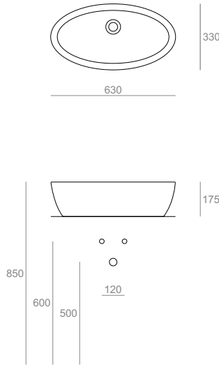
LFT64 Lavabo 63 ovale d'appoggio Oval counter top washbasin 63 63.33.17,5
