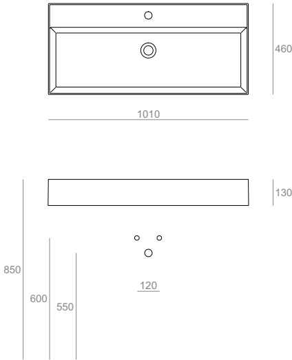
AG101 Lavabo 101 monoforo da appoggio o sospeso Countertop or wall-hung washbasin 101 for single tap hole 101.46.13
