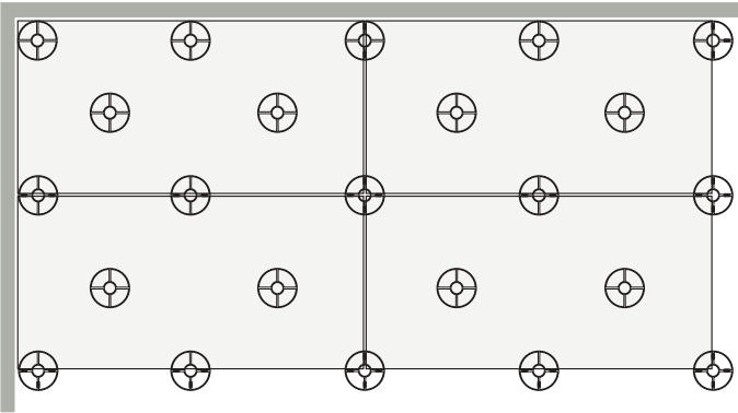
Posa sopraelevata 60×120 \pm 2 cm 24"x48" \pm 3/4" Installation onto flat surfaces (raised laying)
