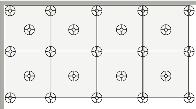
Posa sopraelevata 60×60 \pm 2 cm 24"x24" \pm 3/4" Installation onto flat surfaces (raised laying)
